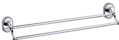
FA-32248 Double towel bar
