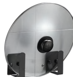
FA-BK5711 Pot cover holder
